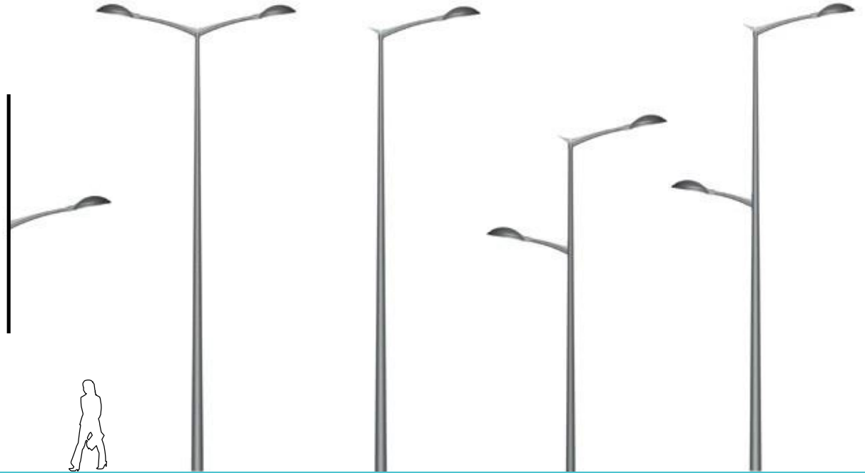
A - Wall mounting B - Kima 800 C - Kima 800 D - Kima 600 E - Kima 800
