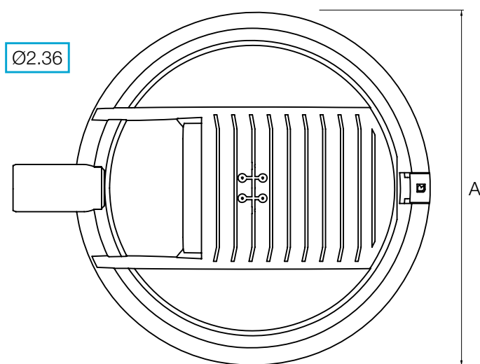
Side mounted
